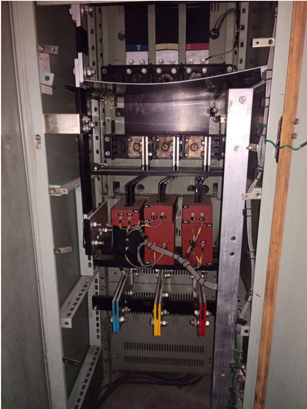
Back view of Panel
